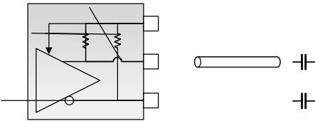
AC-Coupled CML without VCM
