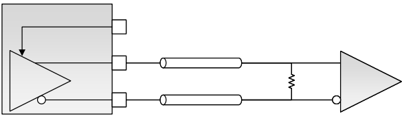
DC-Coupled LVDS
